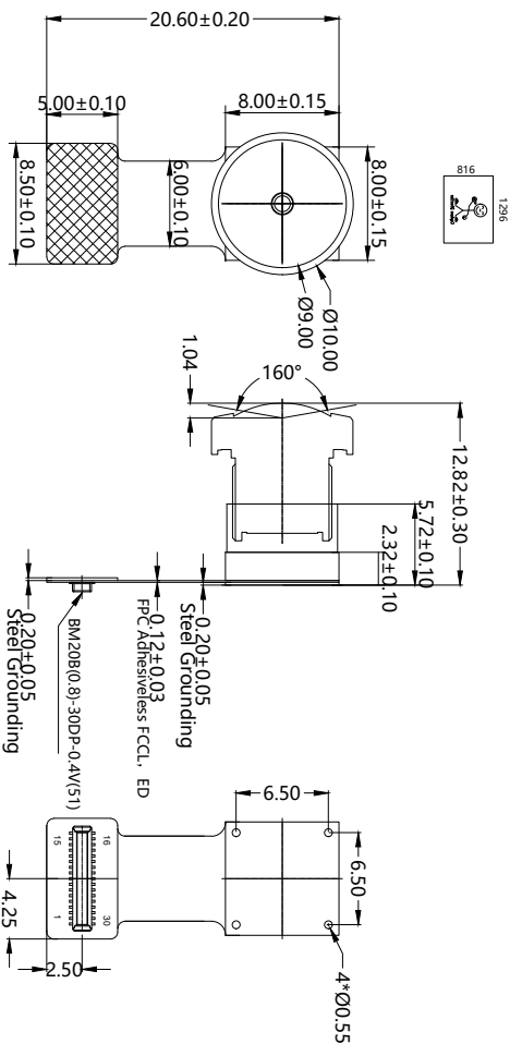
TOP VIEW
